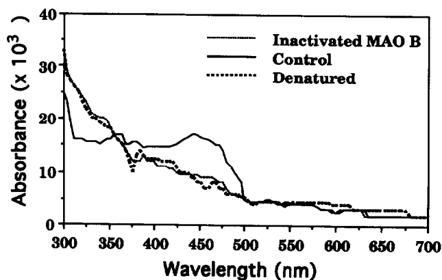
Figure 1. UV-vis spectra before (—) and after (.....) inactivation of MAO by 1 and after denaturation of the inactivated enzyme (----).
