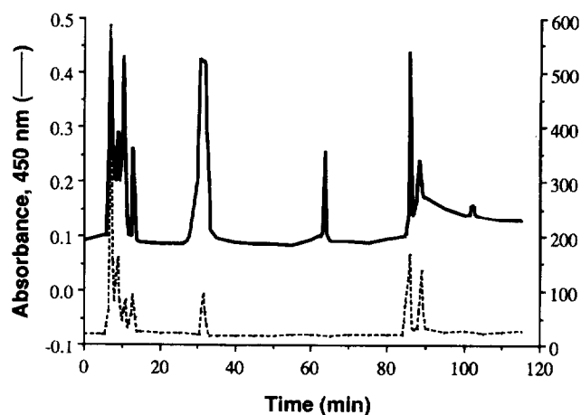
Figure 2. HPLC of the tryptic digest after inactivation of MAO by 8 .
